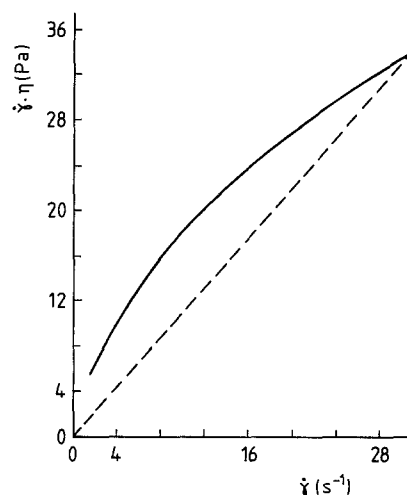
Fig. 1. \eta \dot{\gamma} vs \dot{\gamma} for the solution of 2.5 ml polymethylmetacrylate in 100 ml dimethylphthalate (Lodge 1964). Here \eta is the viscosity coefficient, \dot{\gamma} is the shearing deformation velocity gradient. The \dot{\gamma} value is proportional to the velocity when a body moves in a medium, \eta \dot{\gamma} is proportional to the friction force. The non-linear pattern of the dependence shows the non-Newtonian rheology and the non-linearity of the friction-velocity dependence
